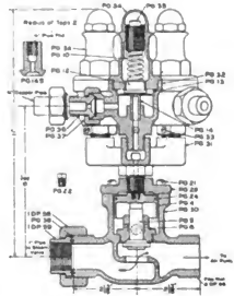
Fig. 2566. 1-Inch Triple Pump Governor.
